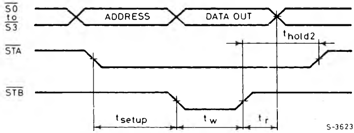
Fig. 3 - Read timing
