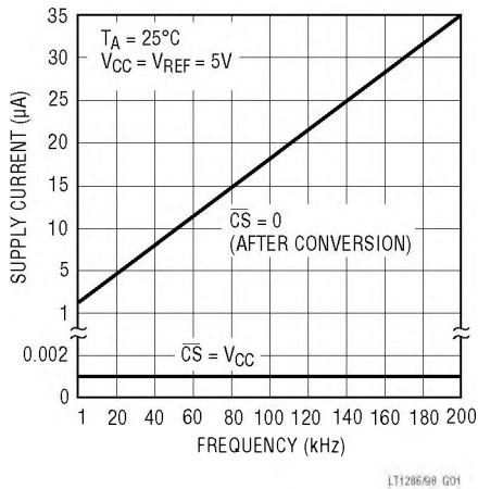
Figure 5. Shutdown current with \overline{CS} high is 1nA typically, regardless of the clock. Shutdown current with \overline{CS} = \text{ground} varies from 1µA at 1kHz to 35µA at 200kHz.
