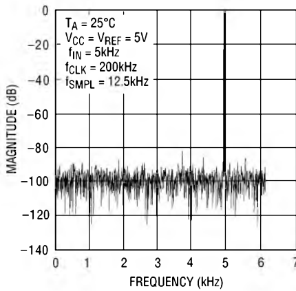
4096 Point FFT Plot
