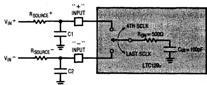
Figure 9. Analog input Equivalent Circuit
