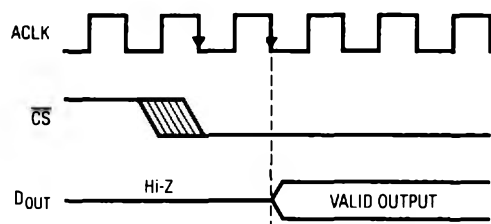
Low \overline{CS} Recognized Internally
