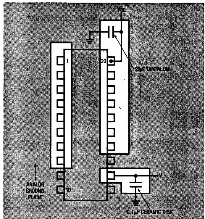
Figure 6. Example Ground Plane for the LTC1290
