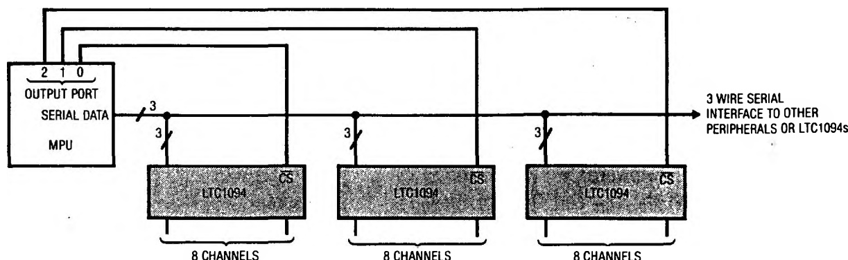
Figure 3. Several LTC1094s Sharing One 3 Wire Serial Interface
