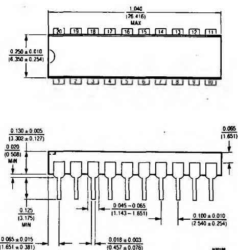
N Package 20 Lead Plastic DIP
