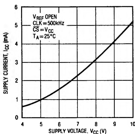
Supply Current vs Supply Voltage LTC1092/3/4
