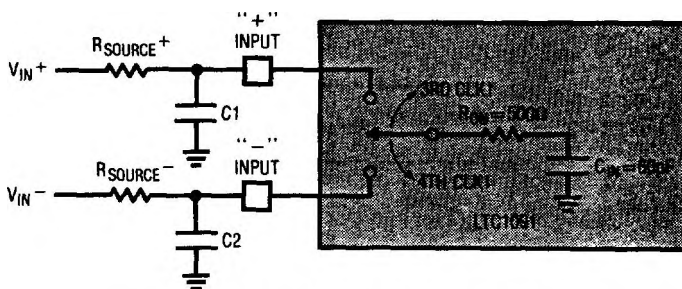
Figure 7. Analog Input Equivalent Circuit
