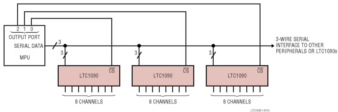
Figure 5. Several LTC1090's Sharing One 3-Wire Serial Interface
