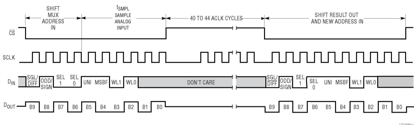
Figure 3. \overline{CS} High During Conversion
