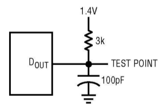
Load Circuit for t dDO , t r , and t f
