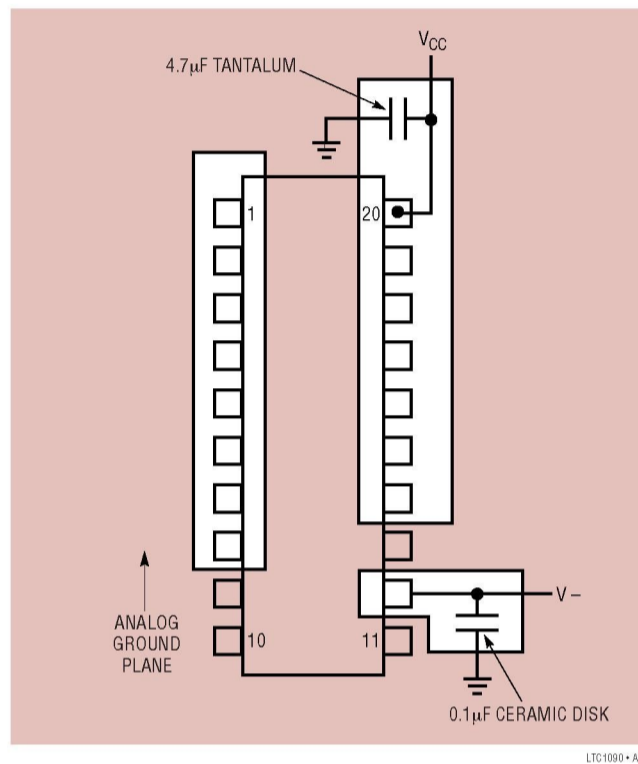
Figure 6. Example Ground Plane for the LTC1090
