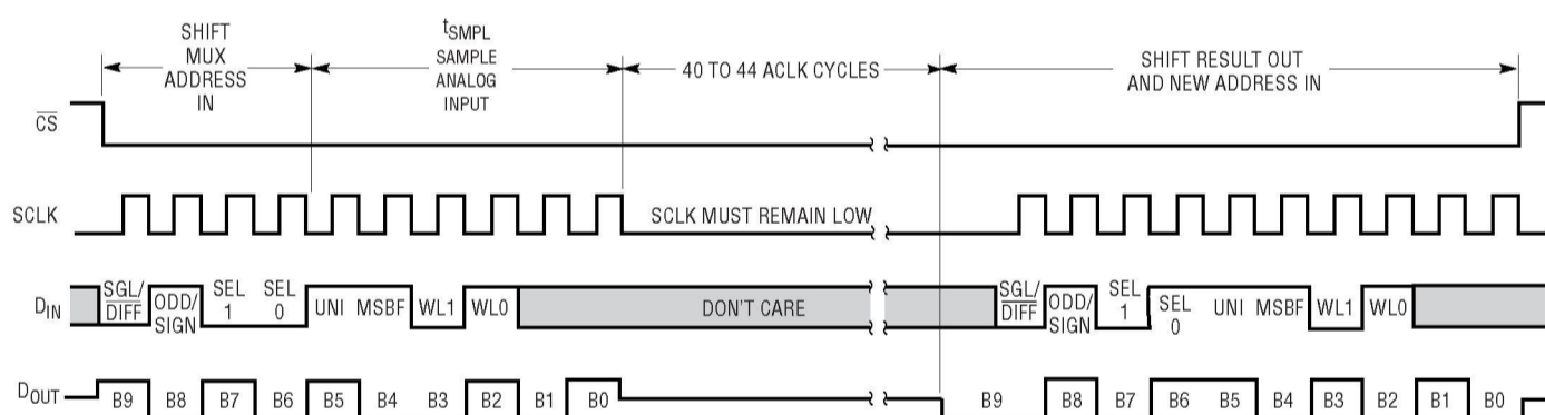
Figure 4. \overline{CS} Low During Conversion
