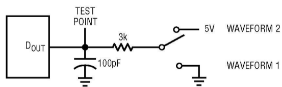
Load Circuit for t dis and t en
