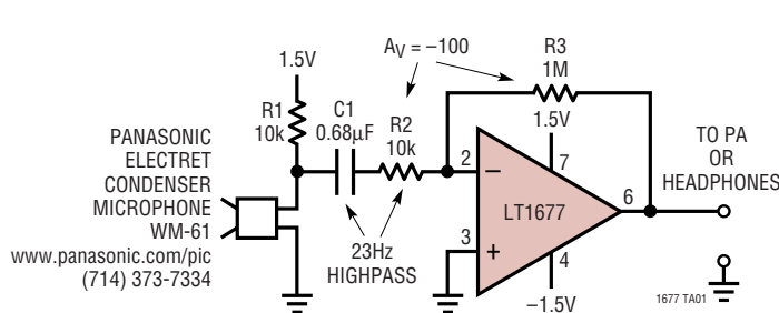
3V Electret Microphone Amplifier
