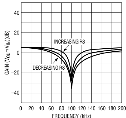
Figure 6. Frequency Response
