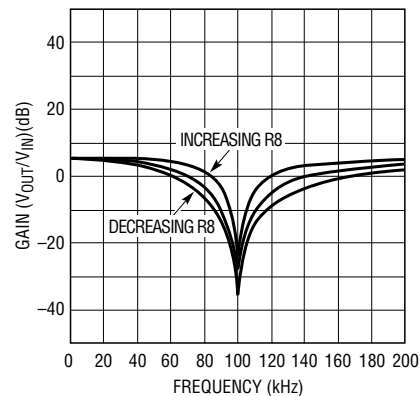
Figure 5. Frequency Response
