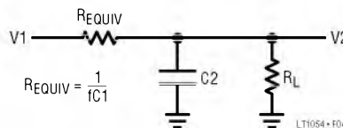
Figure 4. Switched-Capacitor Equivalent Circuit
