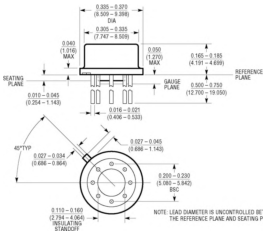
H Package 8-Lead TO-5 Metal Can
