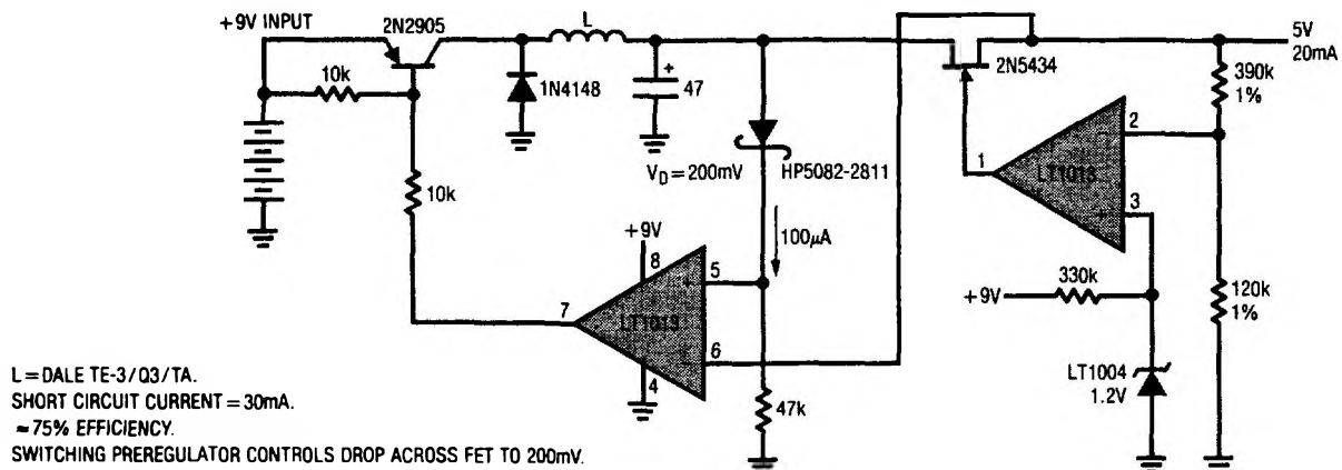
Low Power 9V to 5V Converter
