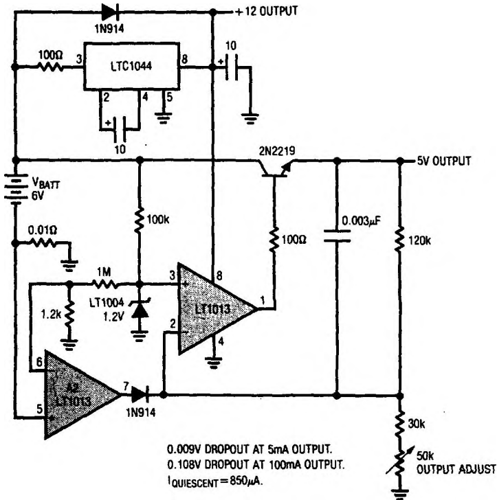
Low Dropout Regulator for 6V Battery
