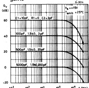
Fig. 18 - Frequency response for various closed loop gains
