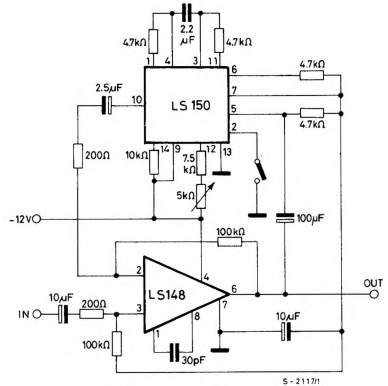
Fig. 2 - Compressor circuit
