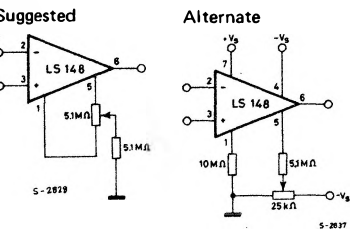
Fig. 1 - Voltage offset null circuit
