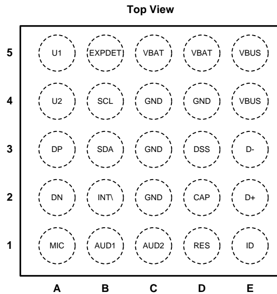
Figure 1. 25-Bump (0.4mm Pitch) DSBGA Package
