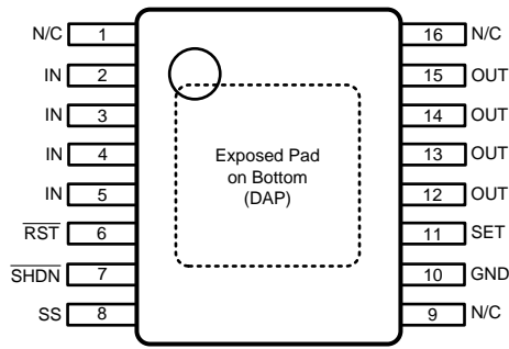
Figure 1. Top View
