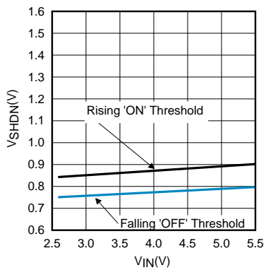
SHDN Thresholds vs V_{IN}
