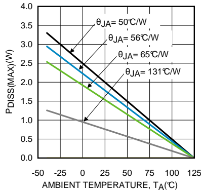
Figure 7. Maximum Dissipation vs. Ambient Temperature
