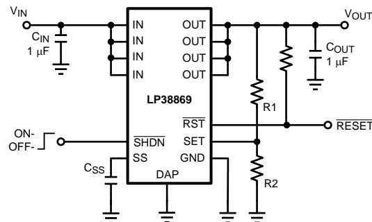
Figure 4. Typical Operating Circuit Adjustable Output Voltage
