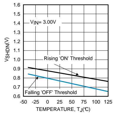
SHDN Thresholds vs Temperature ( T_J )
