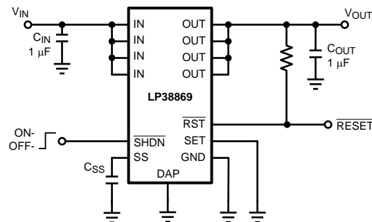
Figure 3. Typical Operating Circuit with Preset Output Voltage
