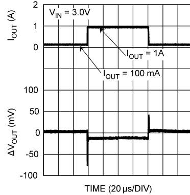
Load Transient Response, V_{IN} = 3.0\text{V}
