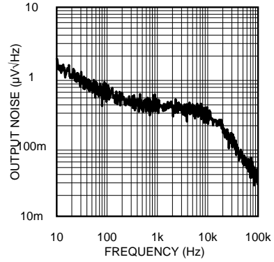
Output Noise Density
