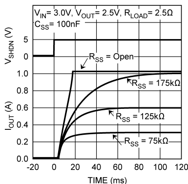
Figure 6. Typical Soft-Start Current Limit Behavior with C_{SS} = 100 \text{ nF}
