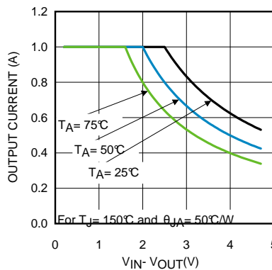
Figure 8. Maximum Output Current vs Input-Output Differential Voltage
