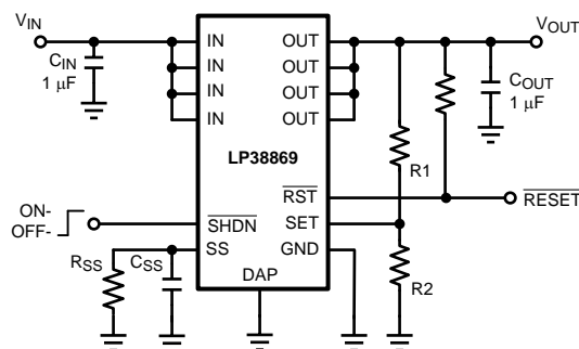
Figure 5. Typical Operating Circuit Soft-Start and Current Limit Reduction
