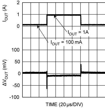
Load Transient Response, V_{IN} = 5.0\text{V}
