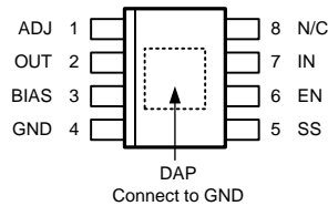
Figure 3. PSOP-8, Top View
