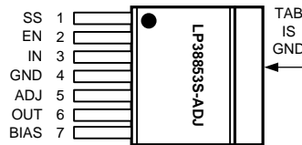
Figure 1. TO263-7, Top View
