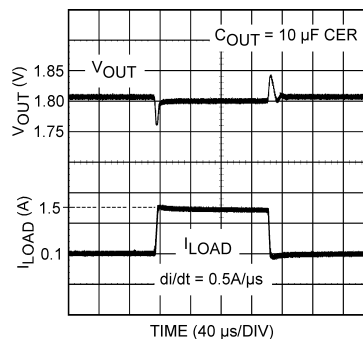
Figure 14. Load Transient Response
