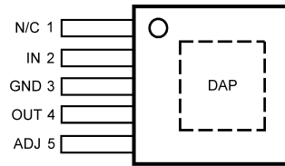
Figure 3. Top View (LP38500TJ-ADJ, LP38500ATJ-ADJ) TO-263 THIN Package
