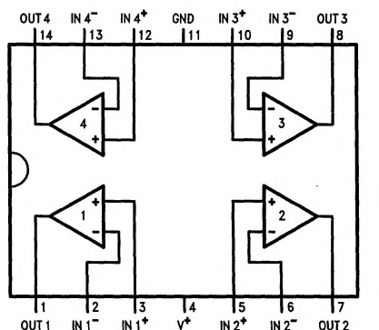
Dual-in-Line (J, N) and SO (M)
