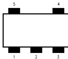
Figure 1. Top View SOT-23, 5-Lead Small Outline Package (M5) Package Number MF05A
