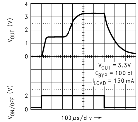
Turn-On Time
