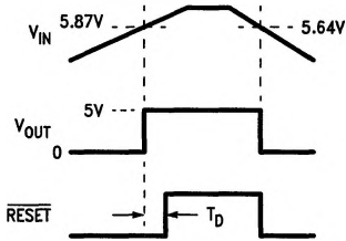
Timing Diagram
