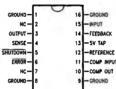
LP2953 16-Pin SO
