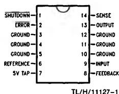
LP2952 14-Pin DIP
