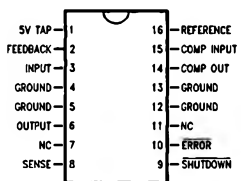
LP2953 16-Pin DIP
