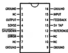
LP2952 16-Pin SO
