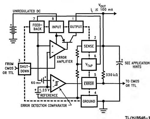
LP2951/A-XX
