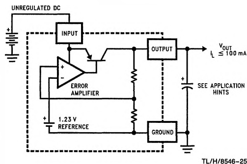
LP2950/A-XX
