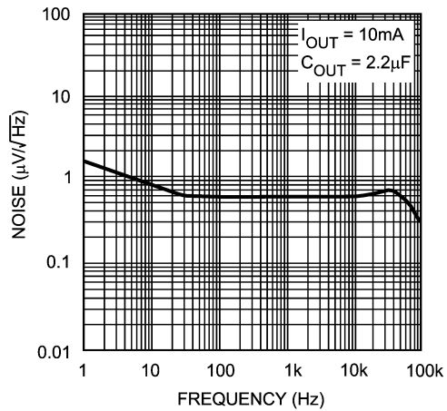
Noise Characteristics
