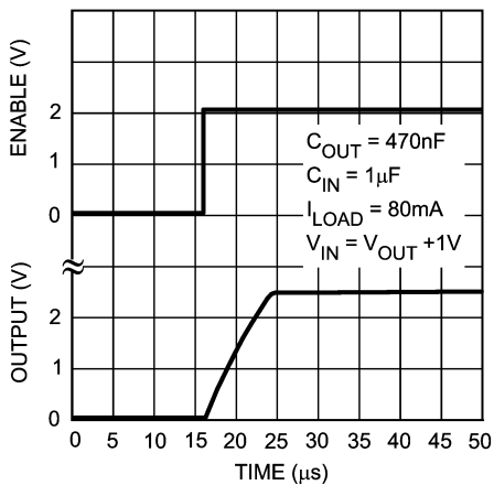
Enable Characteristics
