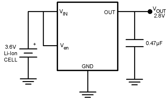
FIGURE 2. Single-Cell Regulator
