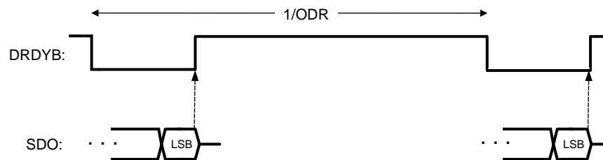
Figure 20. DRDYB Behavior for a Complete ADC_DOUT Reading
