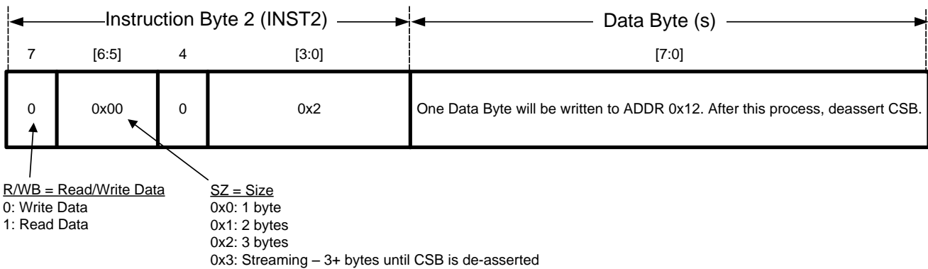
Figure 33. Register-Write Example 2
