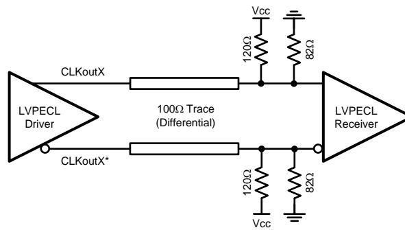
Figure 35. Differential LVPECL Operation, DC Coupling, Thevenin Equivalent
