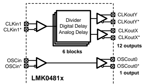
Figure 5. Simplified Functional Block Diagram for Mode Clock Distribution
