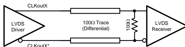
Figure 33. Differential LVDS Operation, DC Coupling, No Biasing of the Receiver
