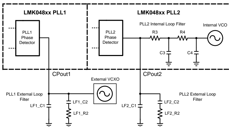
Figure 23. PLL1 and PLL2 Loop Filters
