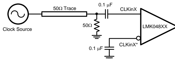
Figure 31. CLKinX/X* Single-ended Termination
