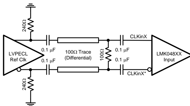
Figure 29. CLKinX/X* Termination for an LVPECL Reference Clock Source
