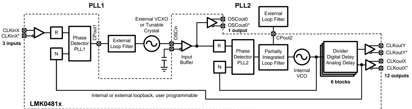
Figure 2. Simplified Functional Block Diagram for 0-delay Dual Loop Mode
