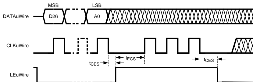
Figure 10. MICROWIRE Timing Diagram: Extra CLKuWire Pulses for R0 to R5 with L Eu Wire Asserted
