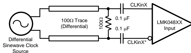
Figure 30. CLKinX/X* Termination for a Differential Sinewave Reference Clock Source
