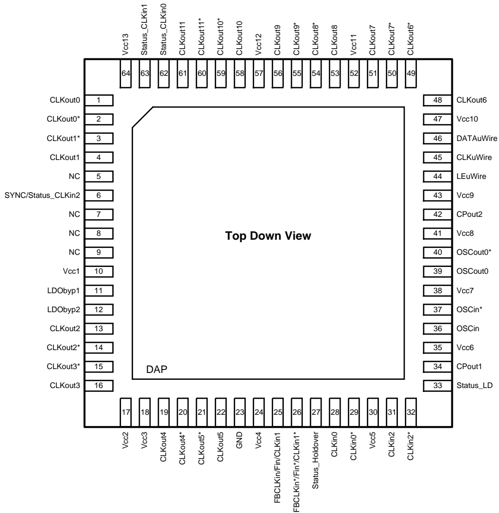
Figure 7. 64-Pin WQFN Package
