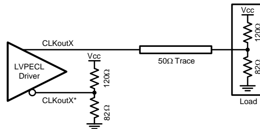
Figure 40. Single-Ended LVPECL Operation, DC Coupling, Thevenin Equivalent
