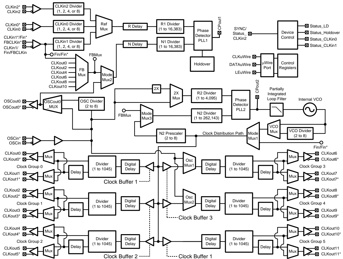
Figure 6. Detailed LMK04816 Block Diagram
