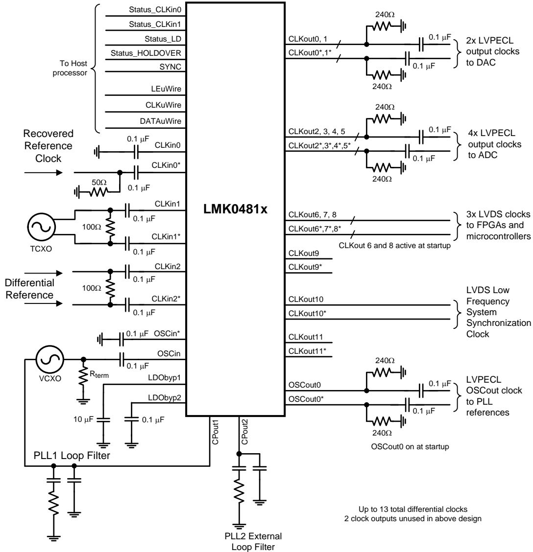
Figure 24. Example Application – System Schematic Except for Power
