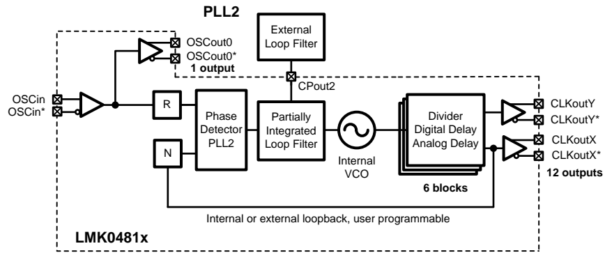
Figure 4. Simplified Functional Block Diagram for 0-delay Single Loop Mode
