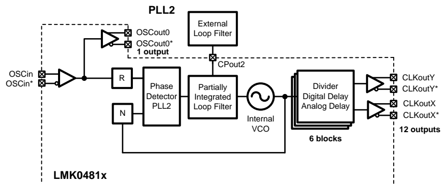
Figure 3. Simplified Functional Block Diagram for Single Loop Mode
