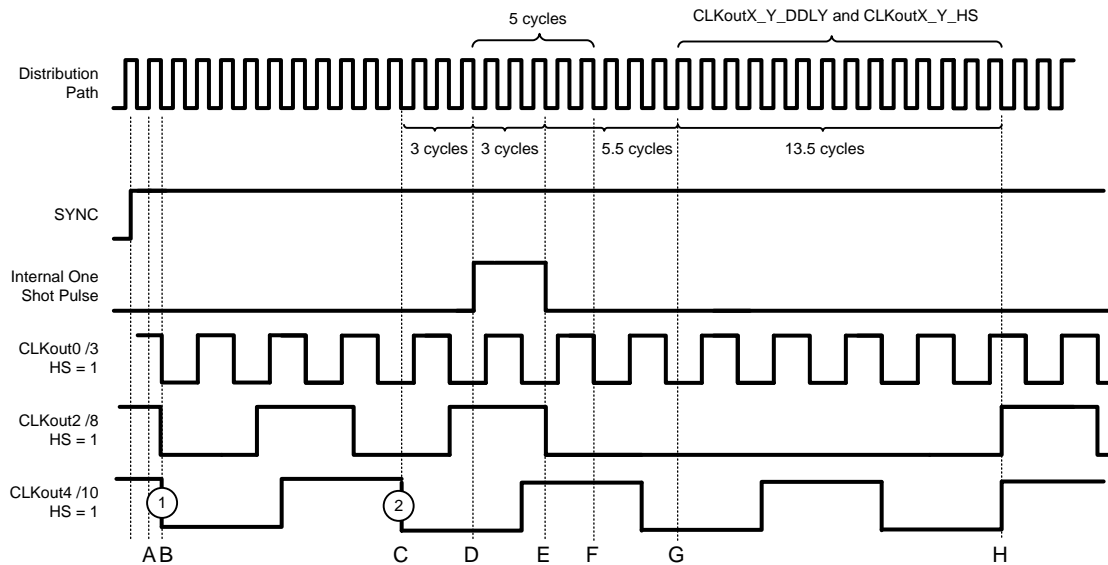
Figure 21. Absolute Dynamic Digital Delay Programming Example (SYNC_QUAL = 1, Qualify with clock output)
