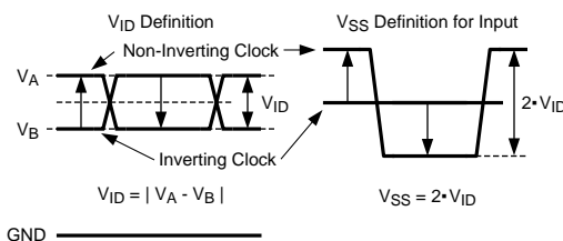
Figure 13. Two Different Definitions for Differential Input Signals
