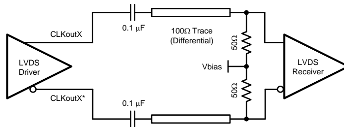
Figure 36. Differential LVDS Operation, AC Coupling, External Biasing at the Receiver
