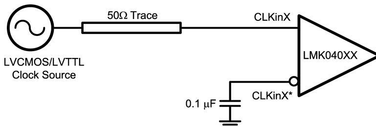
Figure 32. DC Coupled LVCMOS/LVTTL Reference Clock
