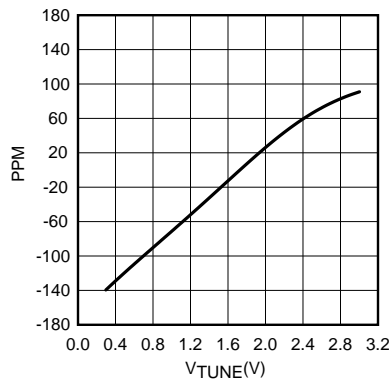
Figure 27. Example Tuning Curve, 20.48 MHz Crystal
