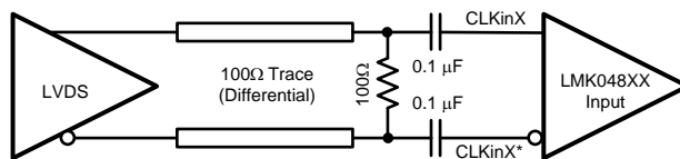
Figure 28. CLKinX/X* Termination for an LVDS Reference Clock Source
