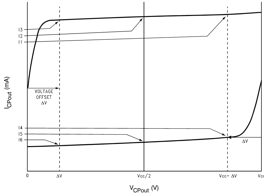
Figure 12. Charge Pump Current
