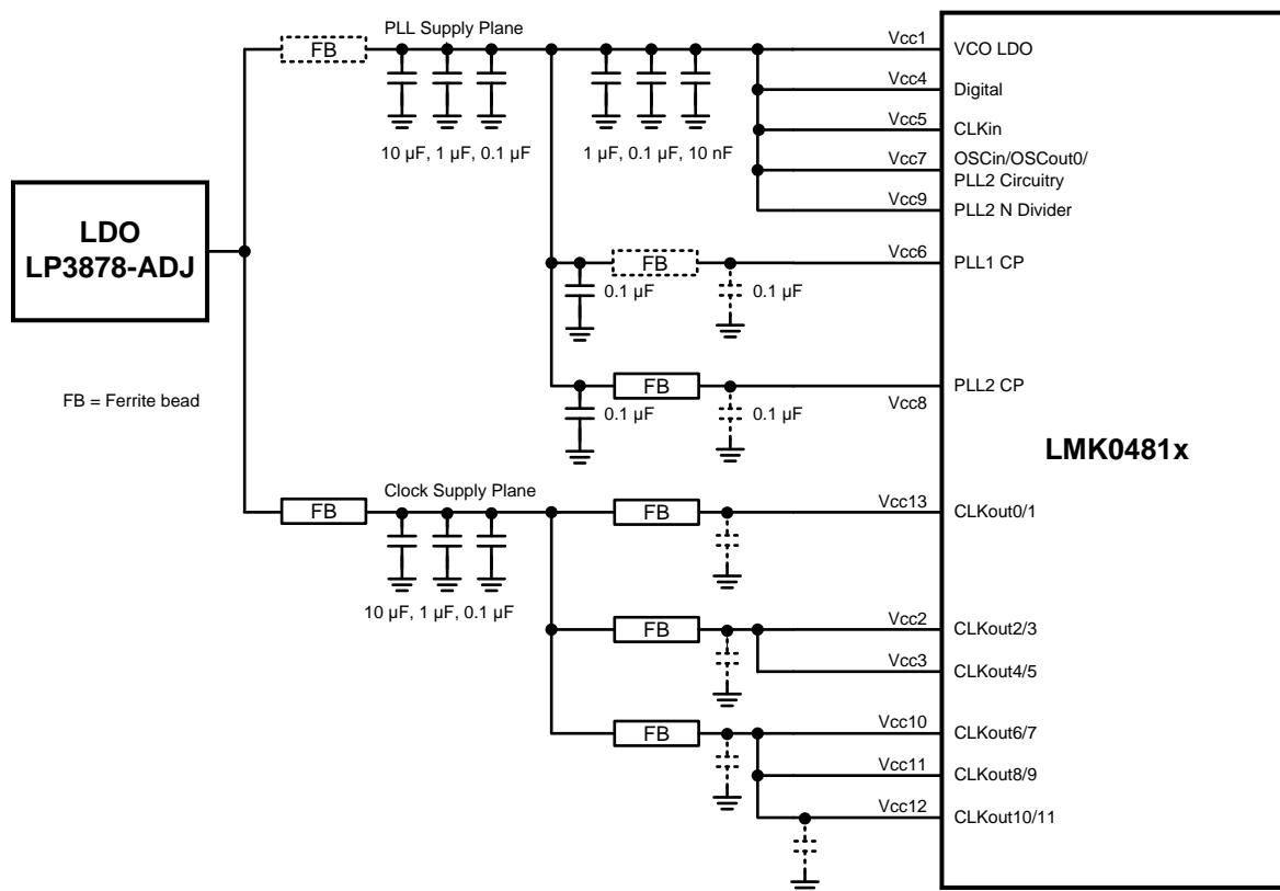
Figure 25. Example Application – Power System Schematic
