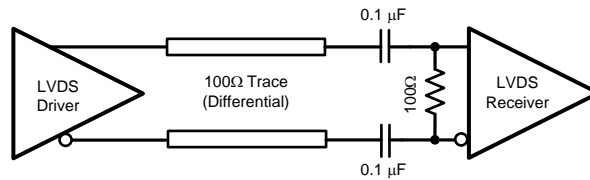
Figure 37. LVDS Termination for a Self-Biased Receiver
