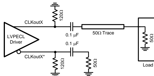
Figure 41. Single-Ended LVPECL Operation, AC Coupling
