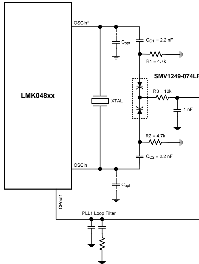
Figure 26. Reference Design Circuit for Crystal Oscillator Option
