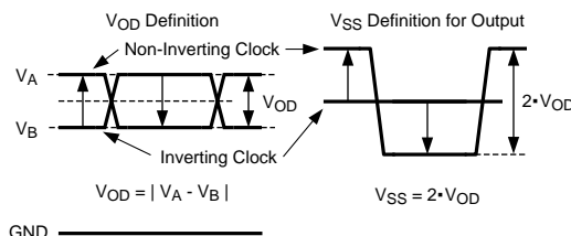
Figure 14. Two Different Definitions for Differential Output Signals
