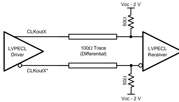
Figure 34. Differential LVPECL Operation, DC Coupling
