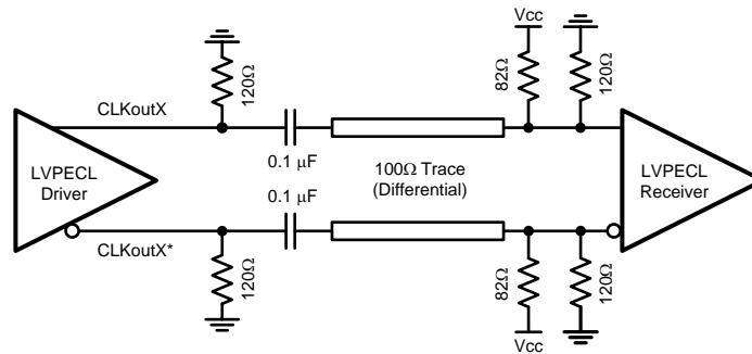
Figure 38. Differential LVPECL Operation, AC Coupling, Thevenin Equivalent, External Biasing at the Receiver
