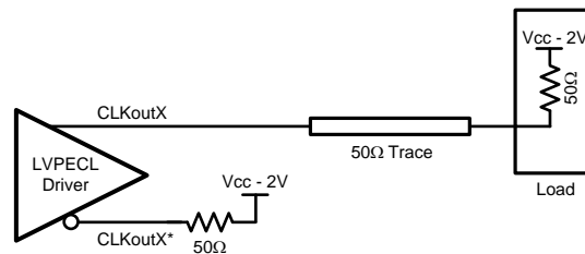
Figure 39. Single-Ended LVPECL Operation, DC Coupling
