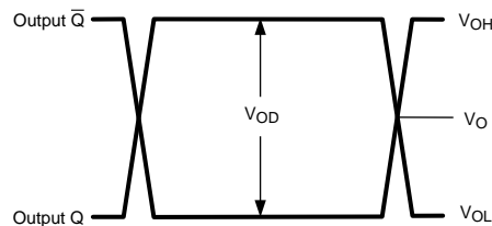
Figure 21. Output Swing
