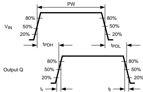
Figure 13. Propagation Delay
