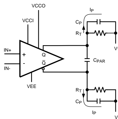
Figure 22. Parasitic Capacitance
