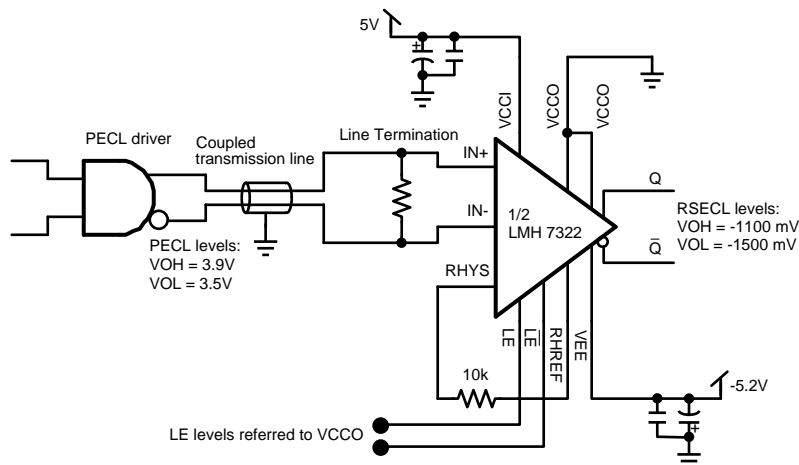
Figure 10. PECL TO RSECL
