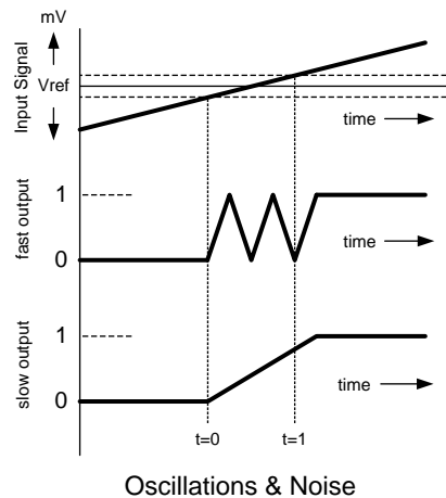
Figure 18. Oscillations on Output Signal
