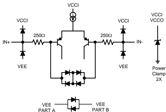
Figure 4. Equivalent Input Circuitry
