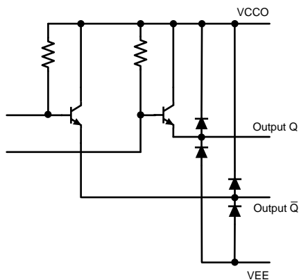
Figure 5. Equivalent Output Circuitry
