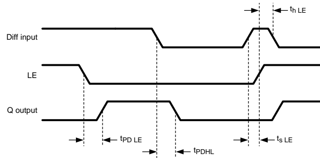
Figure 7. LE Timing
