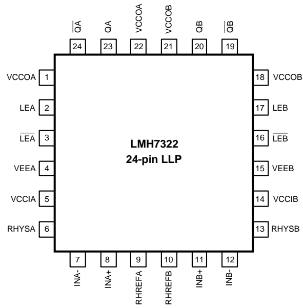
Figure 3. Footprint
