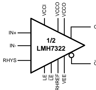
Figure 2. Schematic
