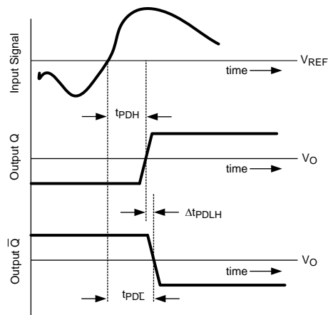
Figure 14. t_{PD} with Complementary Outputs
