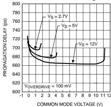
Propagation Delay vs. Common Mode Voltage
