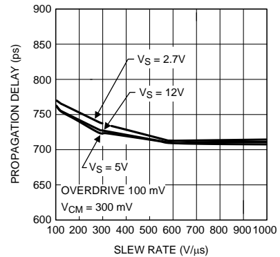
Propagation Delay vs. Slew Rate
