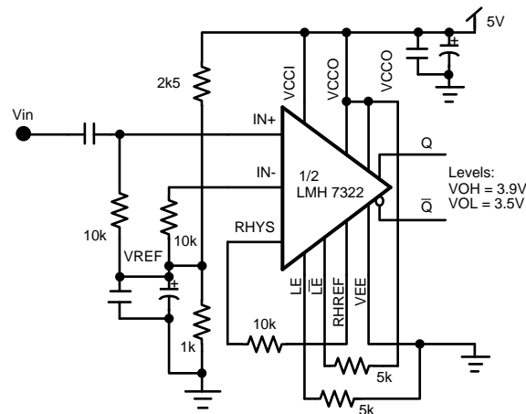
Figure 12. Standard Setup
