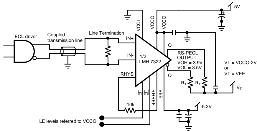
Figure 9. ECL TO RSPECL
