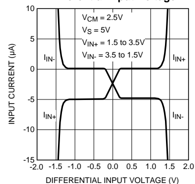
Input Current vs. Differential Input Voltage
