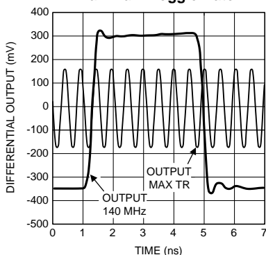
Maximum Toggle Rate
