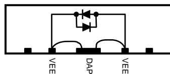
Figure 8. DAP Connection
