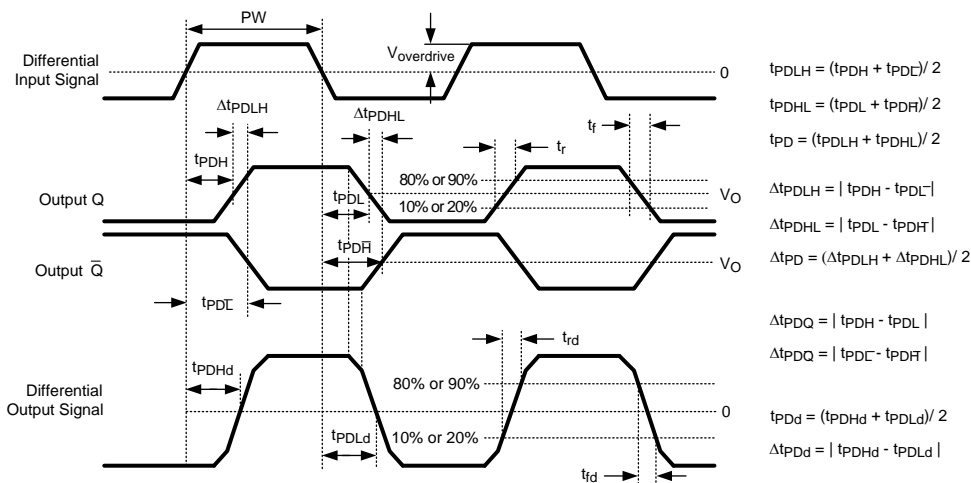
Figure 6. Timing Definitions
