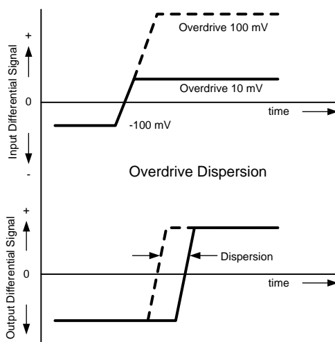
Figure 15. Overdrive Dispersion
