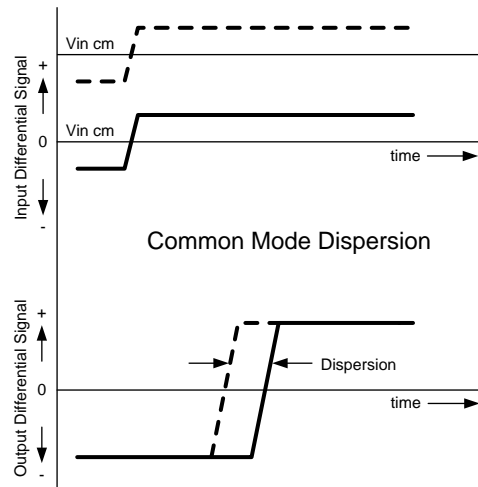
Figure 17. Common Mode Dispersion
