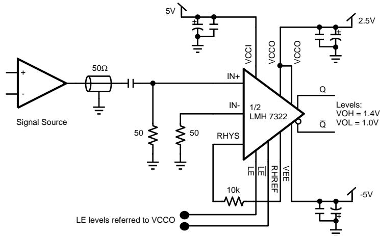
Figure 11. ANALOG TO LVDS
