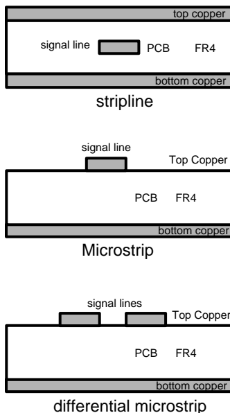
Figure 25. PCB Lines
