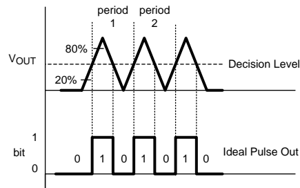
Figure 23. Bit Rates
