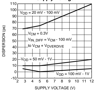
Common Mode Dispersion vs. Supply Voltage
