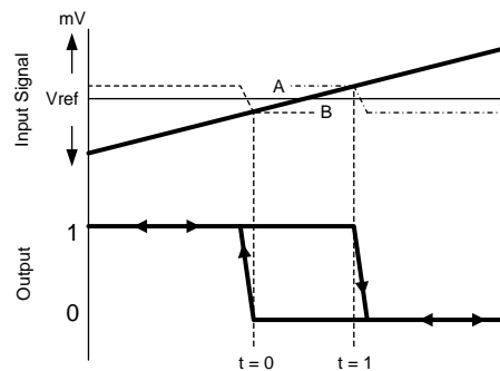
Figure 19. Hysteresis
