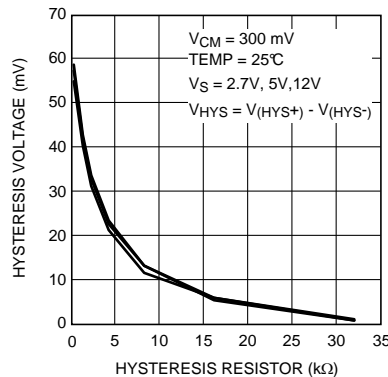
Figure 20. Hysteresis Voltage vs. Hysteresis Resistor
