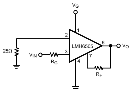
Figure 8. Inverting Amplifier
