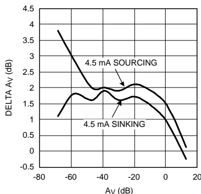
Figure 7. LMH6505 Gain Variation over R_G DC Current Capability vs. Gain
