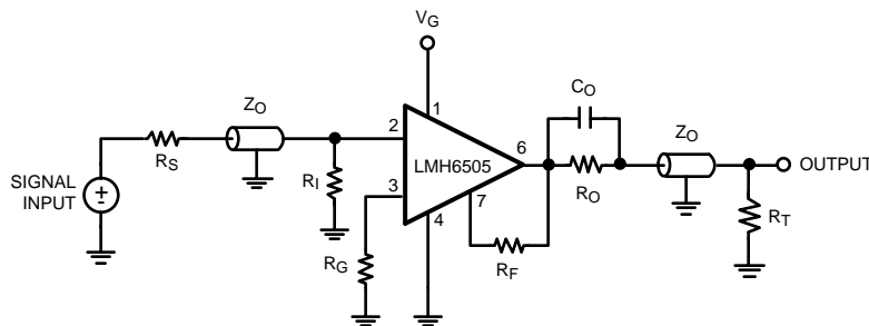
Figure 9. Transmission Line Matching
