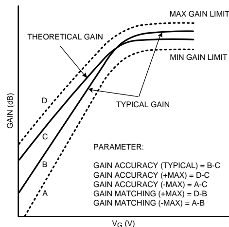
Figure 5. LMH6505 Gain Accuracy & Gain Matching Defined
