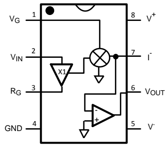
Figure 3. 8-Pin SOIC/MSOP Top View
