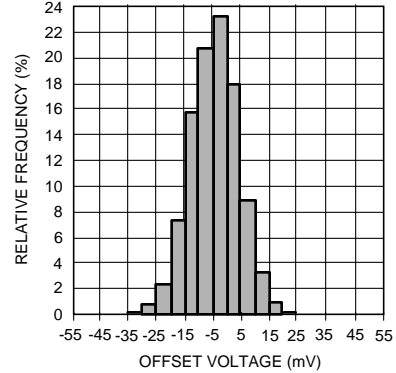
Distribution of Output Offset Voltage
