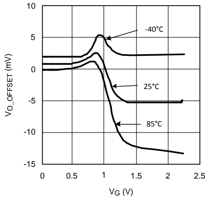
Output Offset Voltage vs. V_G (Typical Unit #3)
