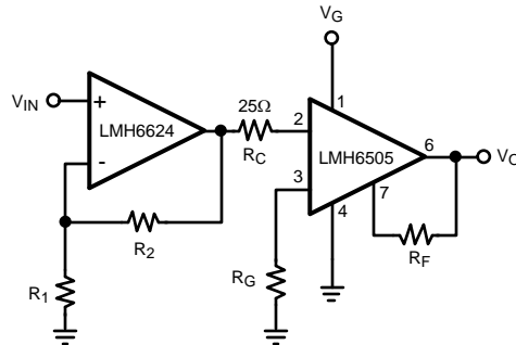
Figure 6. Gain Partitioning
