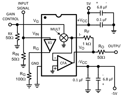
Figure 4. LMH6505 Typical Application and Block Diagram
