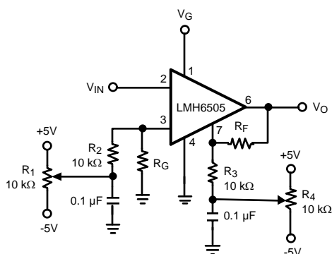
Figure 10. Offset Adjust Circuit
