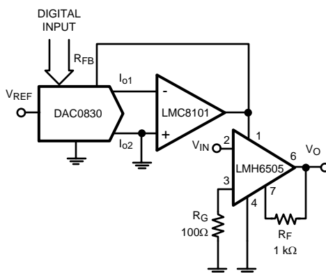
Figure 11. Digital Gain Control
