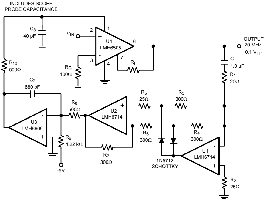
Figure 12. Automatic Gain Control Circuit
