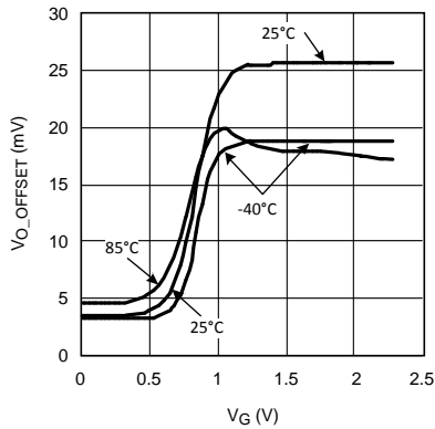
Output Offset Voltage vs. V_G (Typical Unit #3)
