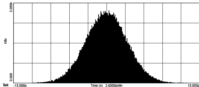
Figure 9. CLKout1 Jitter Histogram Horizontal scale: 2.6ps / division
