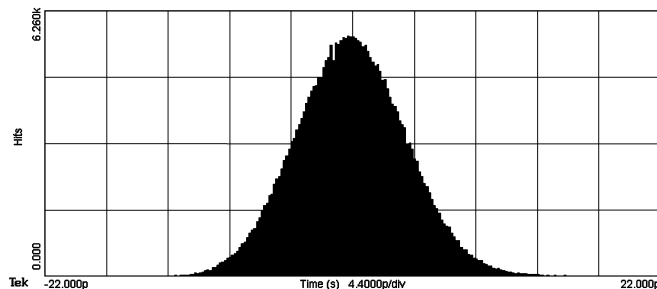
Figure 11. CLKout2 Jitter Histogram Horizontal scale: 4.4ps / division
