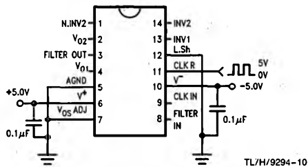
FIGURE 3. Dual Supply Operation LMF60 Driven with TTL Logic Level Clock
