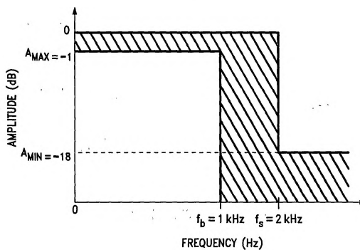
TL/H/10557-17 FIGURE 6. Design Example Magnitude Response Specification. The response of the filter design must fall within the shaded area of the specification.
