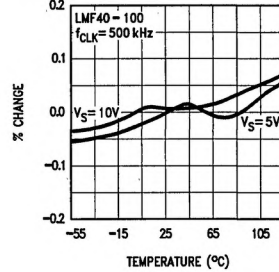
f_{CLK}/f_c Deviation vs Temperature
