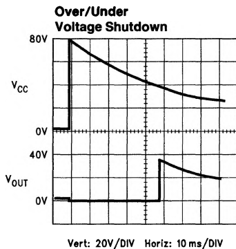
TL/H/11026-12 FIGURE 3. Overvoltage/Undervoltage Shutdown
