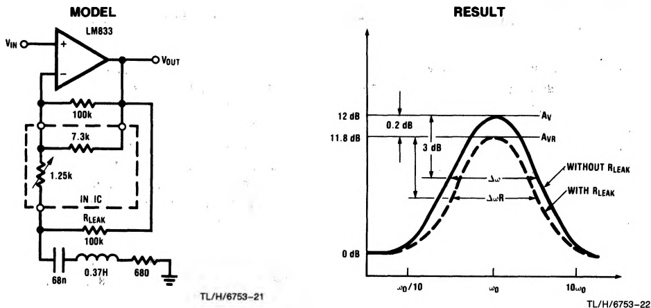
FIGURE 15. Effect of R_{LEAK}
