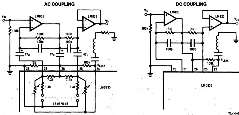
FIGURE 16. Reducing External Components
