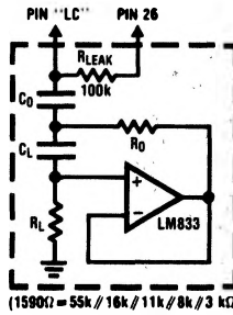
FIGURE 10. Tuned Circuit for 12-Band Equalizer (Figure 9)
