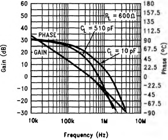
Gain and Phase vs Capacitance Load (2.7V)
