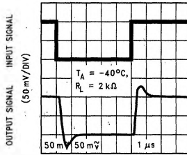
TIME (1 μs/DIV)
