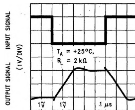
TIME (1 μs/DIV)
