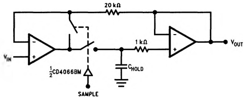
FIGURE 7. Sample and Hold
