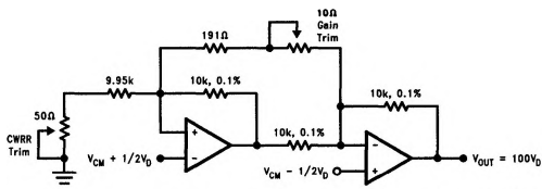
FIGURE 6. Low-Power Two-Op-Amp Instrumentation Amplifier
