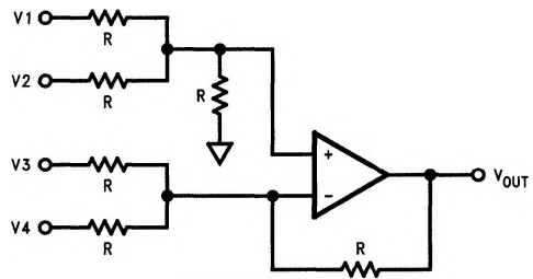
FIGURE 9. Adder/Subtractor Circuit
