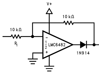
Figure 24. Full Wave Rectifier with Input Current Protection ( R_I )
