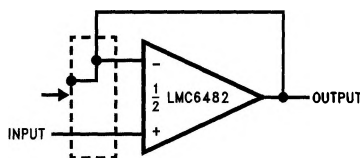
(c) Follower
