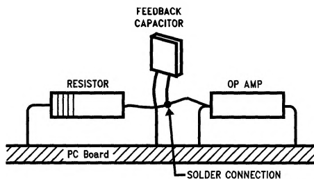
FIGURE 11. Air Wiring
