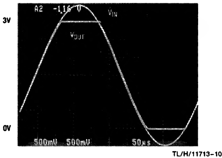
FIGURE 1. An Input Voltage Signal Exceeds the LMC6482 Power Supply Voltages with No Output Phase Inversion
