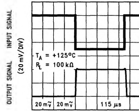
TIME (115 μs/DIV)
