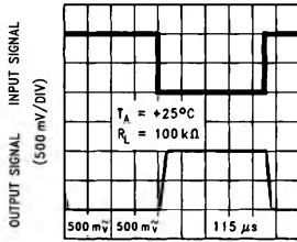
TIME (115 μs/DIV)
