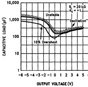
Stability vs Capacitive Load, R_L = 20\ k\Omega
