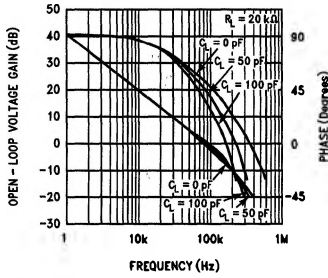
Gain and Phase Response vs Capacitive Load with R_L = 20\ k\Omega
