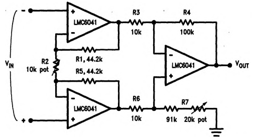
FIGURE 9. Instrumentation Amplifier
