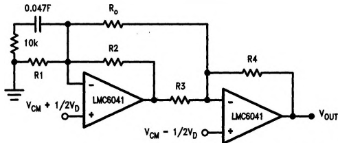
FIGURE 6. Two Op-Amp Instrumentation Amplifier
