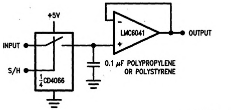
FIGURE 8. Low-Leakage Sample and Hold
