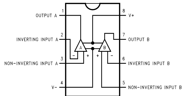
8-Pin PDIP/SOIC Top View
