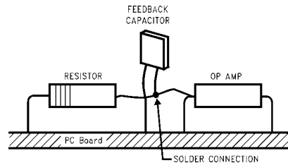
FIGURE 5. Air Wiring
