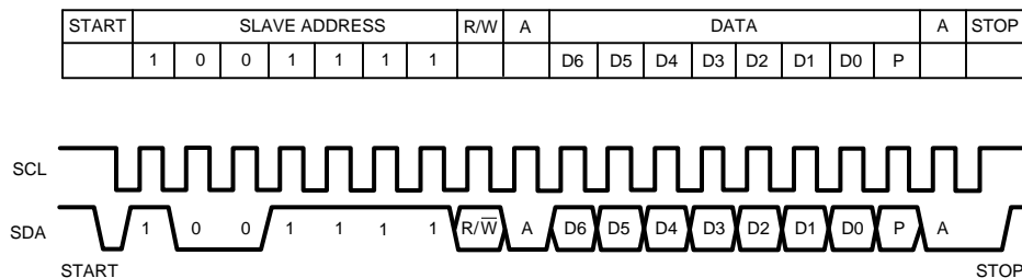
Figure 7. Timing Diagram
