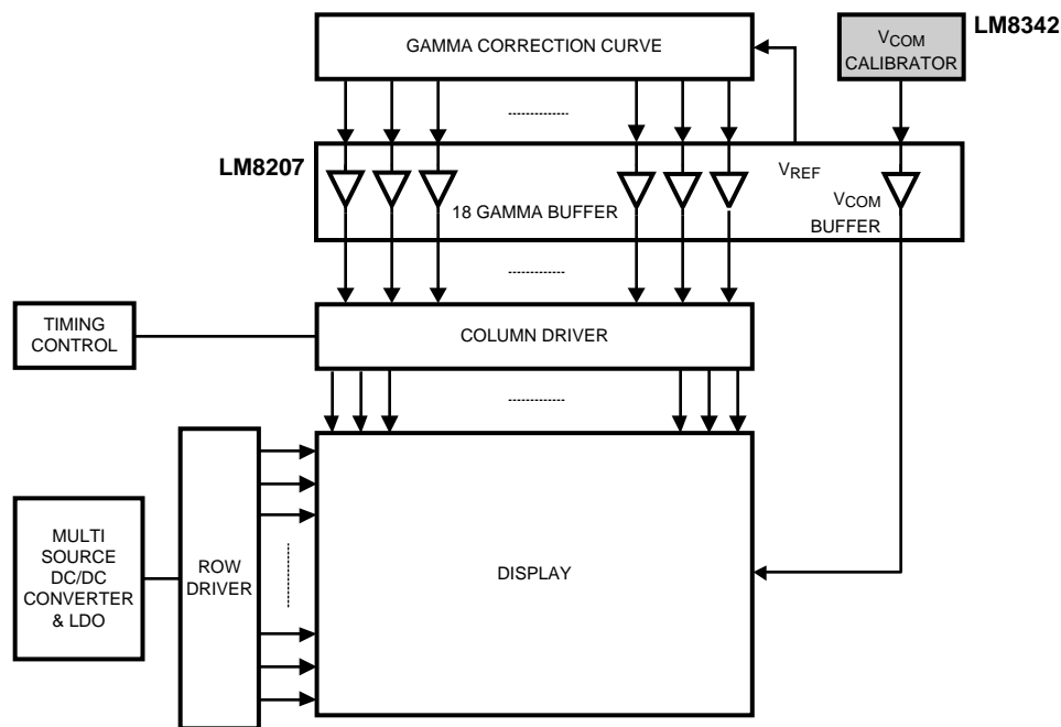
Figure 4. TFT Panel Block Diagram
