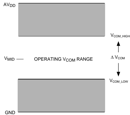
Figure 10. V_{COM} Voltage Levels
