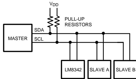
Figure 6. System Using an I 2 C compatible Bus
