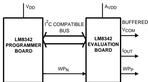
Figure 11. LM8342 Evaluation System
