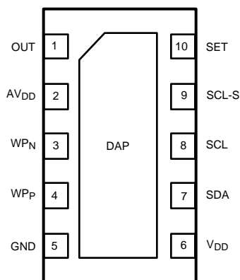
Figure 1. 10-Pin LLP - Top View
