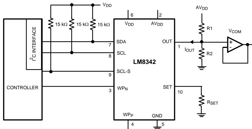
Figure 9. Typical Application Driving a V_{COM} Level
