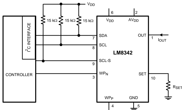
Figure 8. Programmable Current Sink
