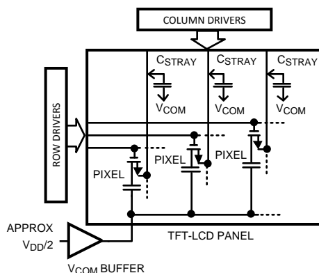
Figure 3. TFT Display
