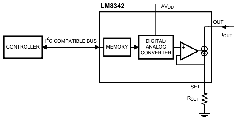
Figure 5. Block Diagram of the LM8342
