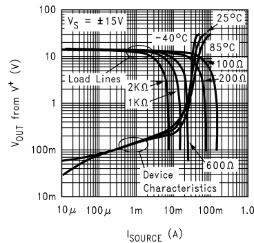
Figure 8. Output Sourcing Characteristics with Load Lines
