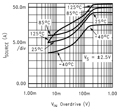
Figure 5. Output Short Circuit Sourcing Current vs. Input Overdrive
