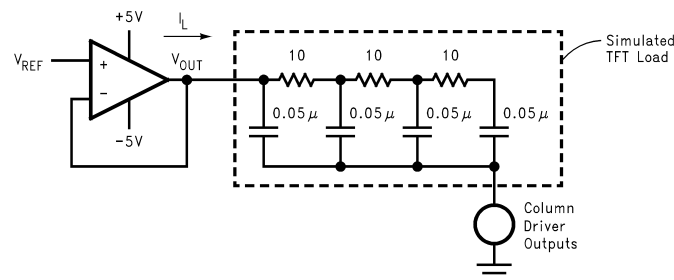
Figure 10. V_{COM} Driver Application Schematic
