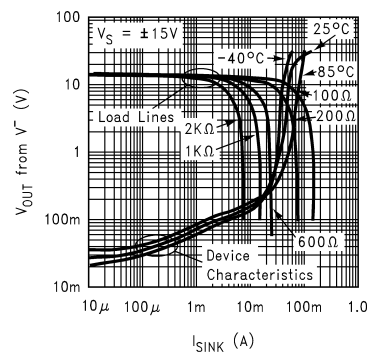
Figure 9. Output Sinking Characteristics with Load Lines
