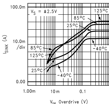
Figure 6. Output Short Circuit Sinking Current vs. Input Overdrive
