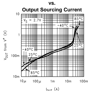
Output Voltage
