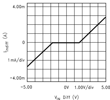
Figure 4. Input Stage Current vs. Differential Input Voltage
