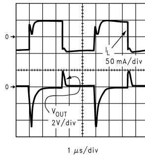
Figure 11. V_{COM} driver performance scope photo
