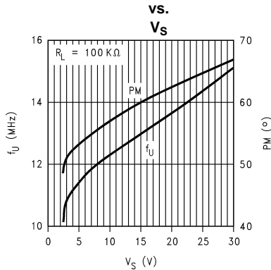
Phase Margin
