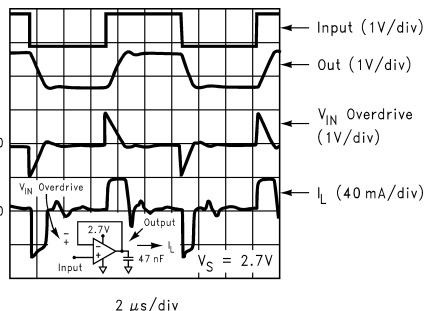
Figure 7. Buffer Amplifier scope photo
