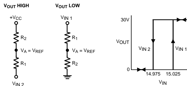
Figure 7. Non-Inverting Comparator with Hysteresis
