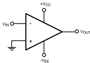
Figure 4. Inverting Comparator
