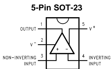
Figure 3. Top View
