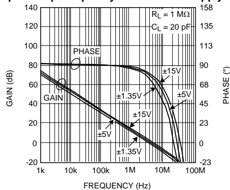
Open Loop Frequency with Various Supply Voltage
