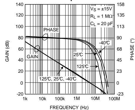
Open Loop Frequency Response with Various Temperatures
