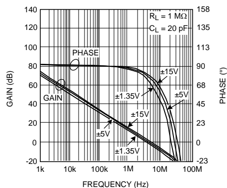
Figure 1. Open Loop Frequency Response
