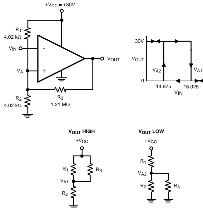
Figure 6. Inverting Comparator with Hysteresis
