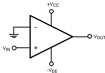
Figure 5. Non-Inverting Comparator
