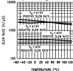
Slew Rate vs Temperature A_V = -1, R_L = 150\Omega
