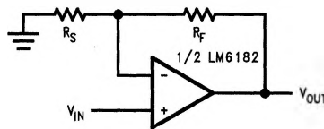
FIGURE 18. Non-Inverting Closed Loop Gain is Determined with the Same Equation Voltage Feedback Amplifiers Use: 1 + R_f/R_s
