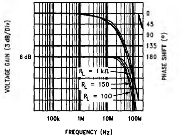
Non-Inverting Gain vs -3 dB Bandwidth R_f = 820\Omega
