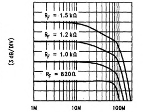
NON-INVERTING GAIN FREQUENCY COMPENSATION V_S = \pm 15\text{V}; A_V = +2; R_L = 150\Omega
