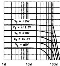
FREQUENCY RESPONSE vs SUPPLY VOLTAGE A_v = -1; R_f = 820\Omega; R_L = 1\text{ k}\Omega
