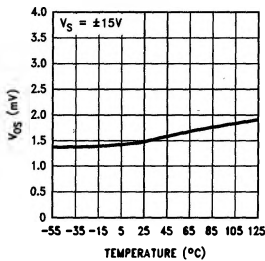
OFFSET VOLTAGE vs TEMPERATURE
