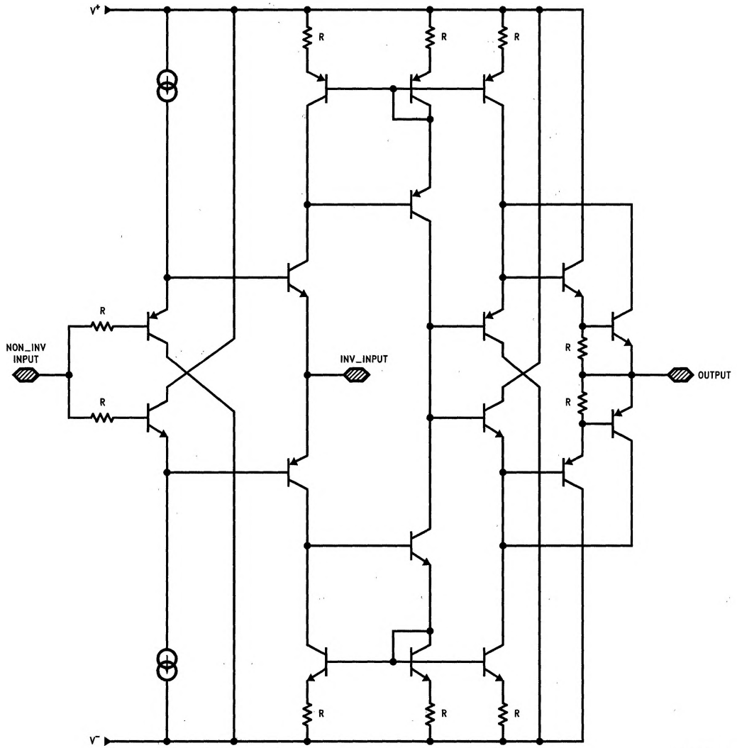
Simplified Schematic
