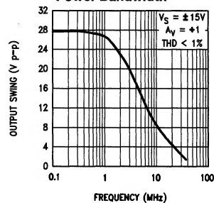
Power Bandwidth
