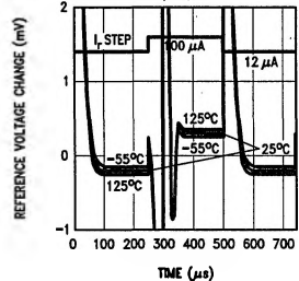
Reference Voltage with 100 ~ 12 \mu\text{A} Current Step
