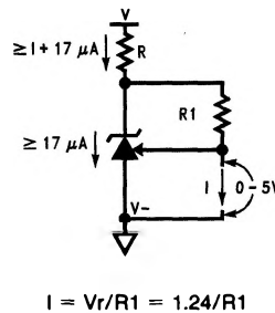
FIGURE 9. Current Source is Programmed by R1
