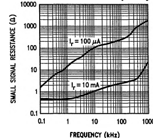
Reference Small-Signal Resistance vs Frequency
