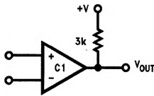
FIGURE 16. Basic Comparator
